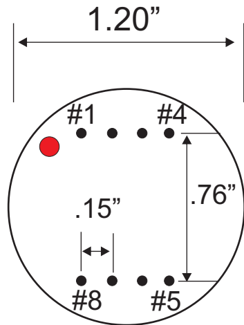
Pin side view
